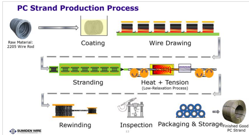
Figure 2. Production process of Stainless steel PC strand
